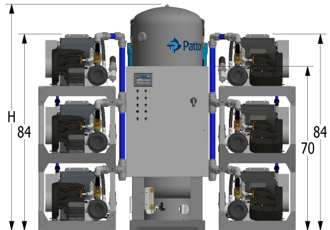
Hexaplex Scroll Medical Air Package Specifications 1
